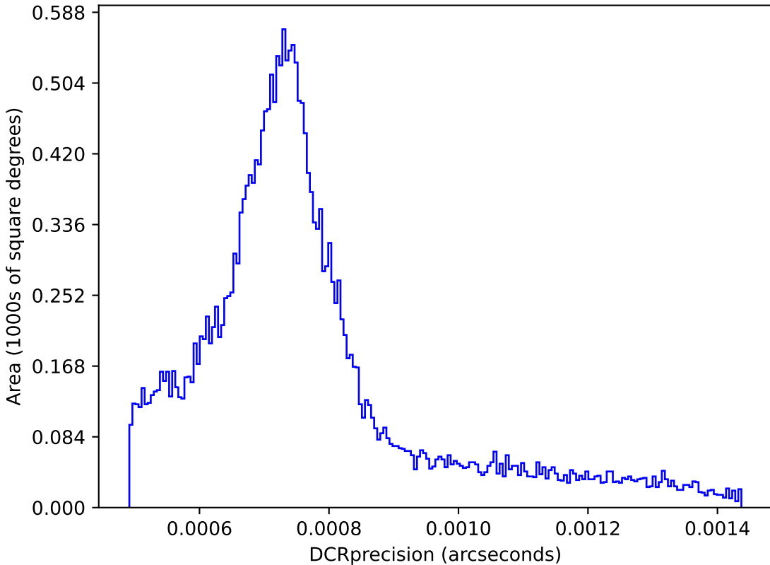
internal_u_expt38_nscale1.1v3.4_10yrs : DCRprecision
