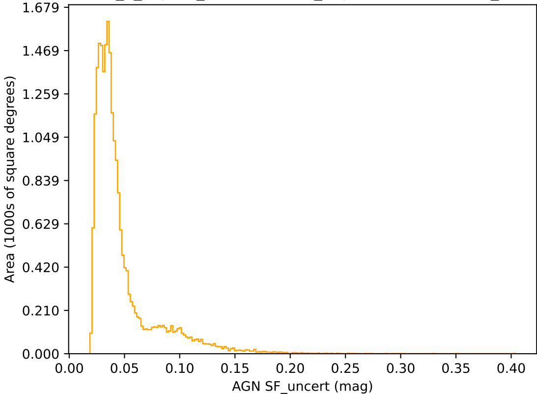
internal_u_expt38_nscale1.1v3.4_10yrs r band: AGN SF_uncert
