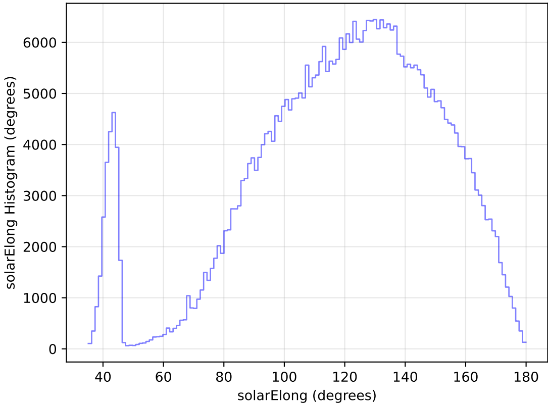
internal_u_expt38_nscale1.1v3.4_10yrs WFD z band: solarElong Histogram
