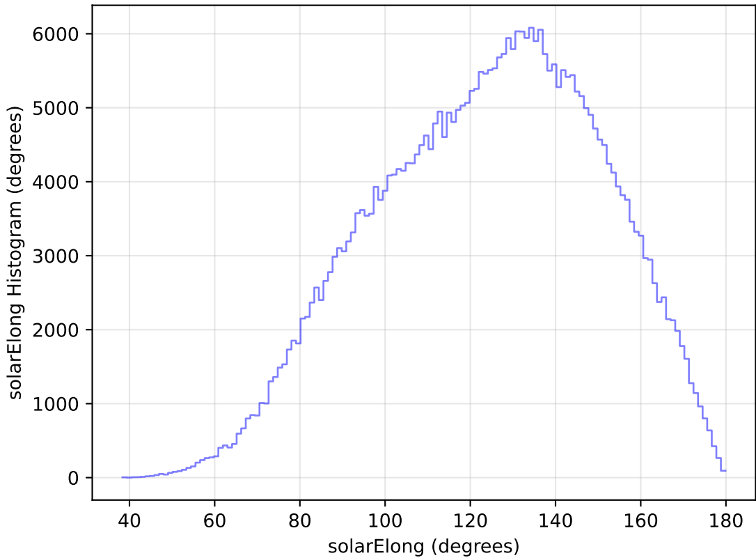
internal_u_expt38_nscale1.1v3.4_10yrs WFD y band: solarElong Histogram
