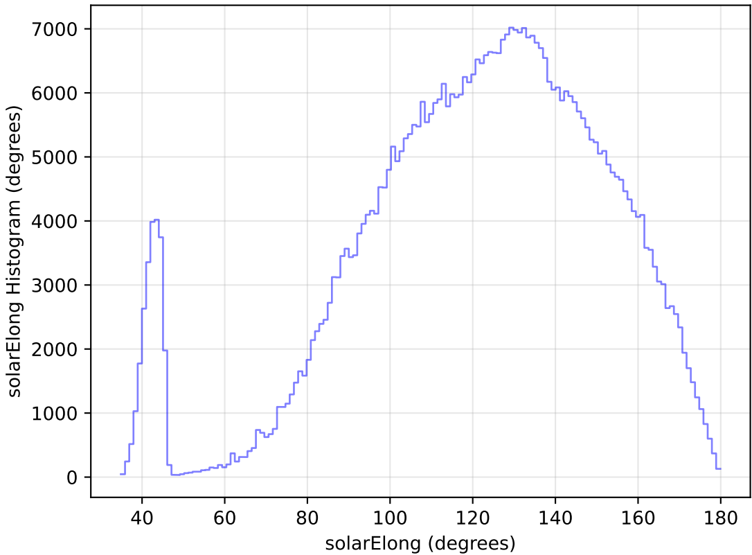
internal_u_expt38_nscale1.1v3.4_10yrs WFD i band: solarElong Histogram
