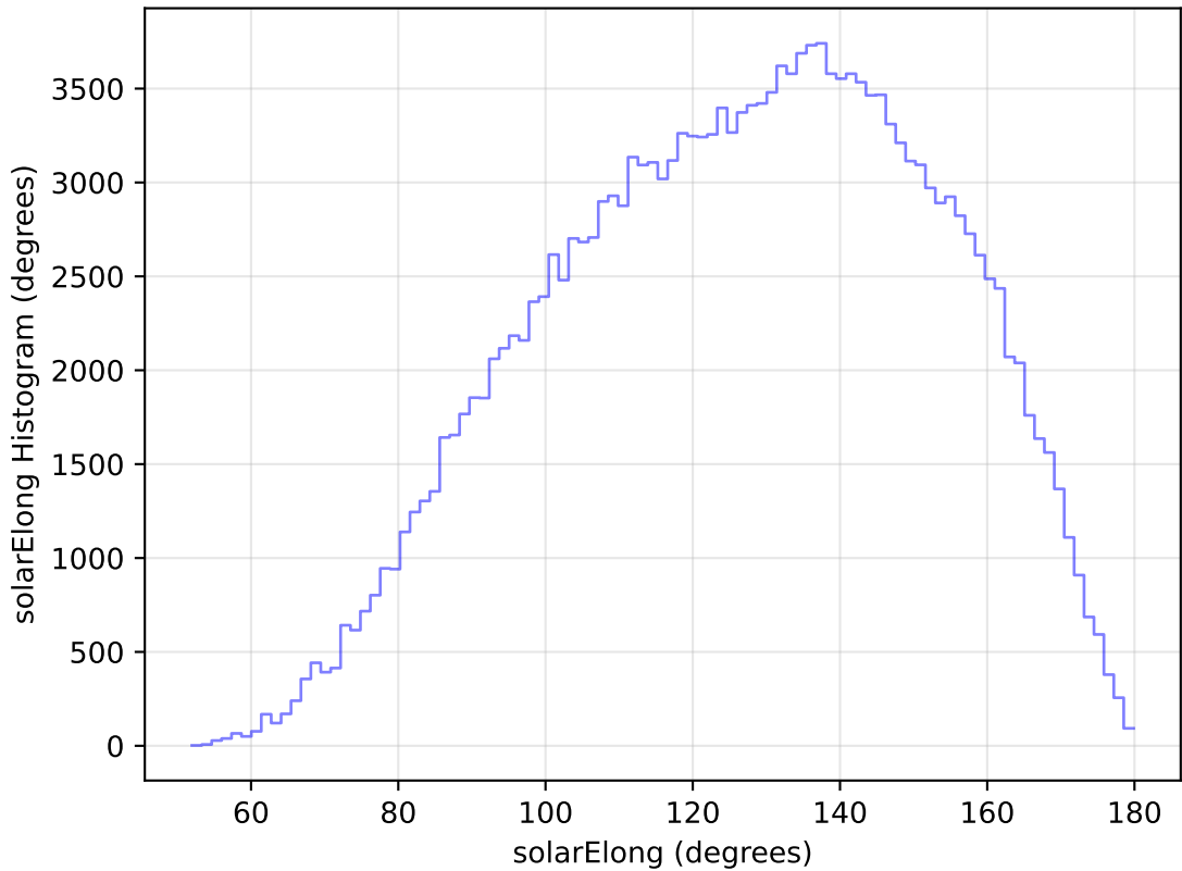
internal_u_expt38_nscale1.1v3.4_10yrs WFD g band: solarElong Histogram
