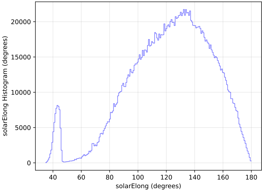
internal_u_expt38_nscale1.1v3.4_10yrs WFD all bands: solarElong Histogram
