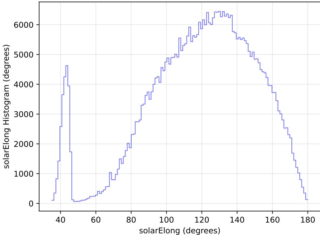
internal_u_expt38_nscale1.1v3.4_10yrs All sky z band: solarElong Histogram
