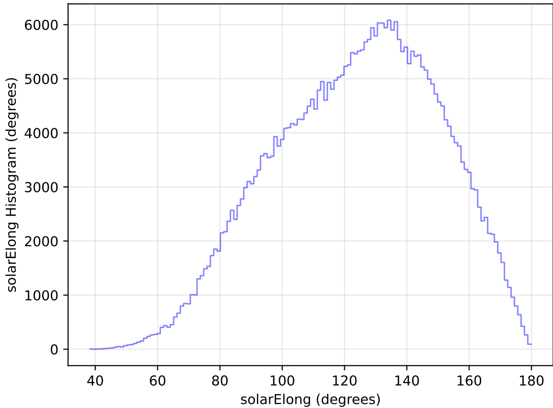
internal_u_expt38_nscale1.1v3.4_10yrs All sky y band: solarElong Histogram
