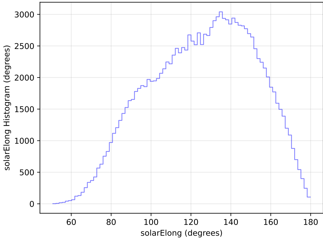
internal_u_expt38_nscale1.1v3.4_10yrs All sky u band: solarElong Histogram
