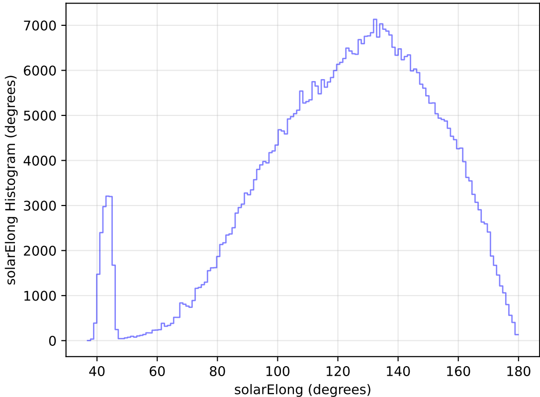
internal_u_expt38_nscale1.1v3.4_10yrs All sky r band: solarElong Histogram
