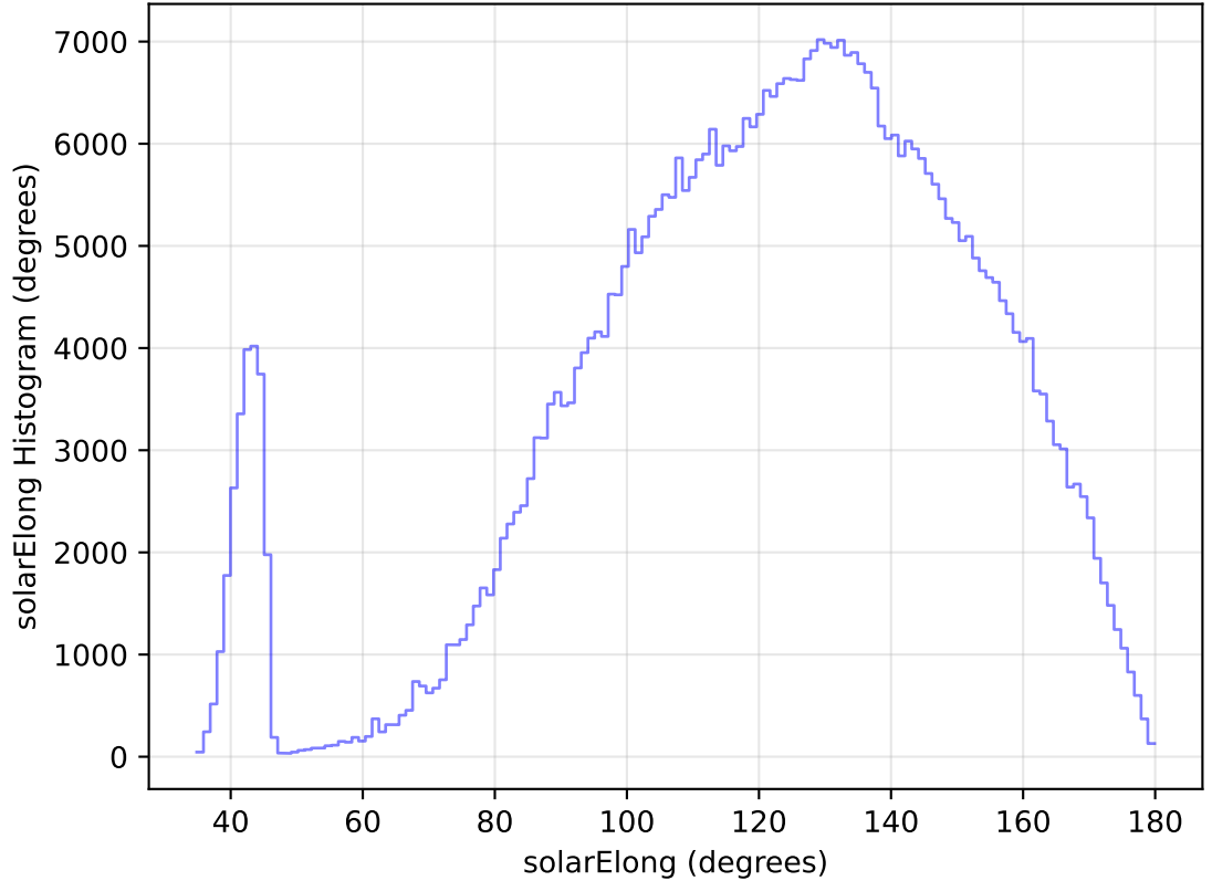
internal_u_expt38_nscale1.1v3.4_10yrs All sky i band: solarElong Histogram
