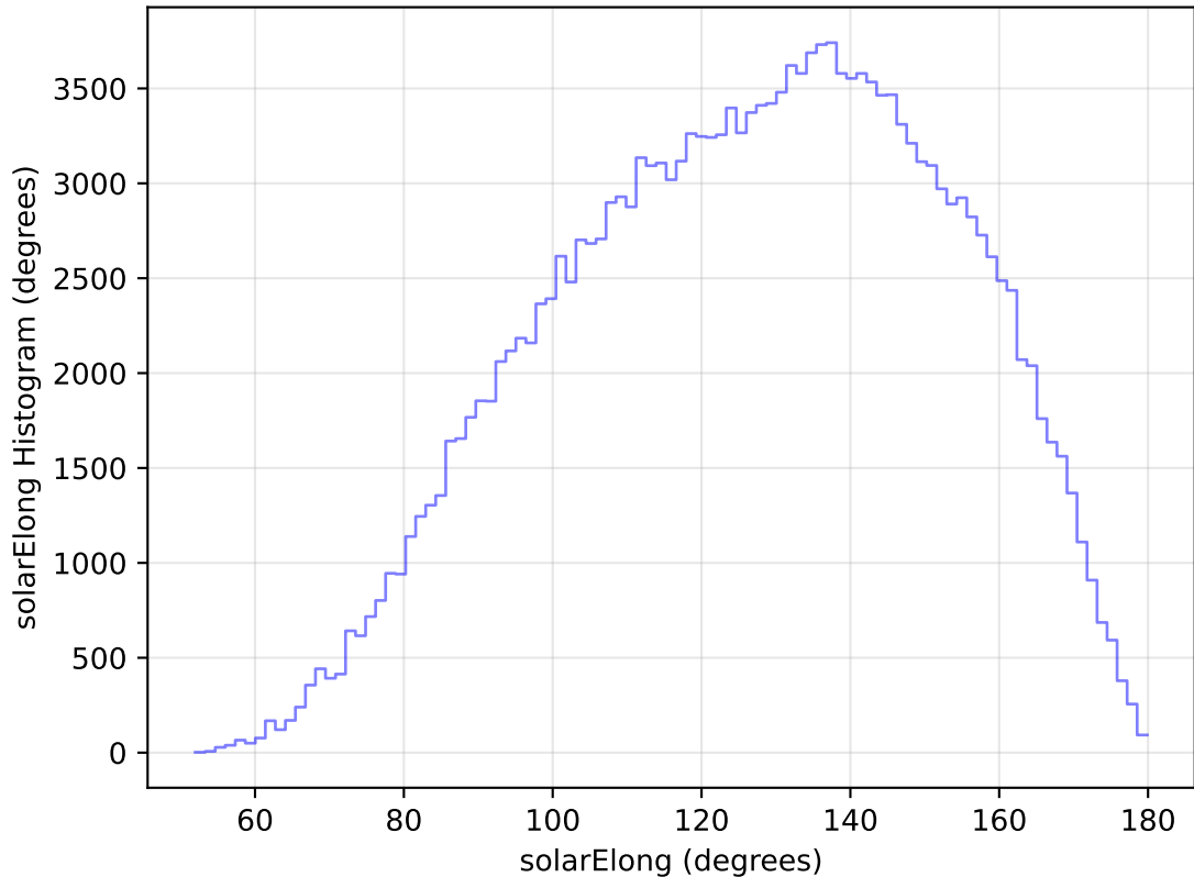
internal_u_expt38_nscale1.1v3.4_10yrs All sky g band: solarElong Histogram
