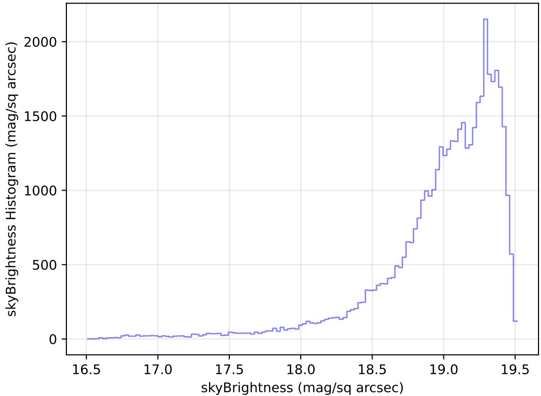
internal_u_expt38_nscale1.1v3.4_10yrs Yr 1 z band: skyBrightness Histogram
