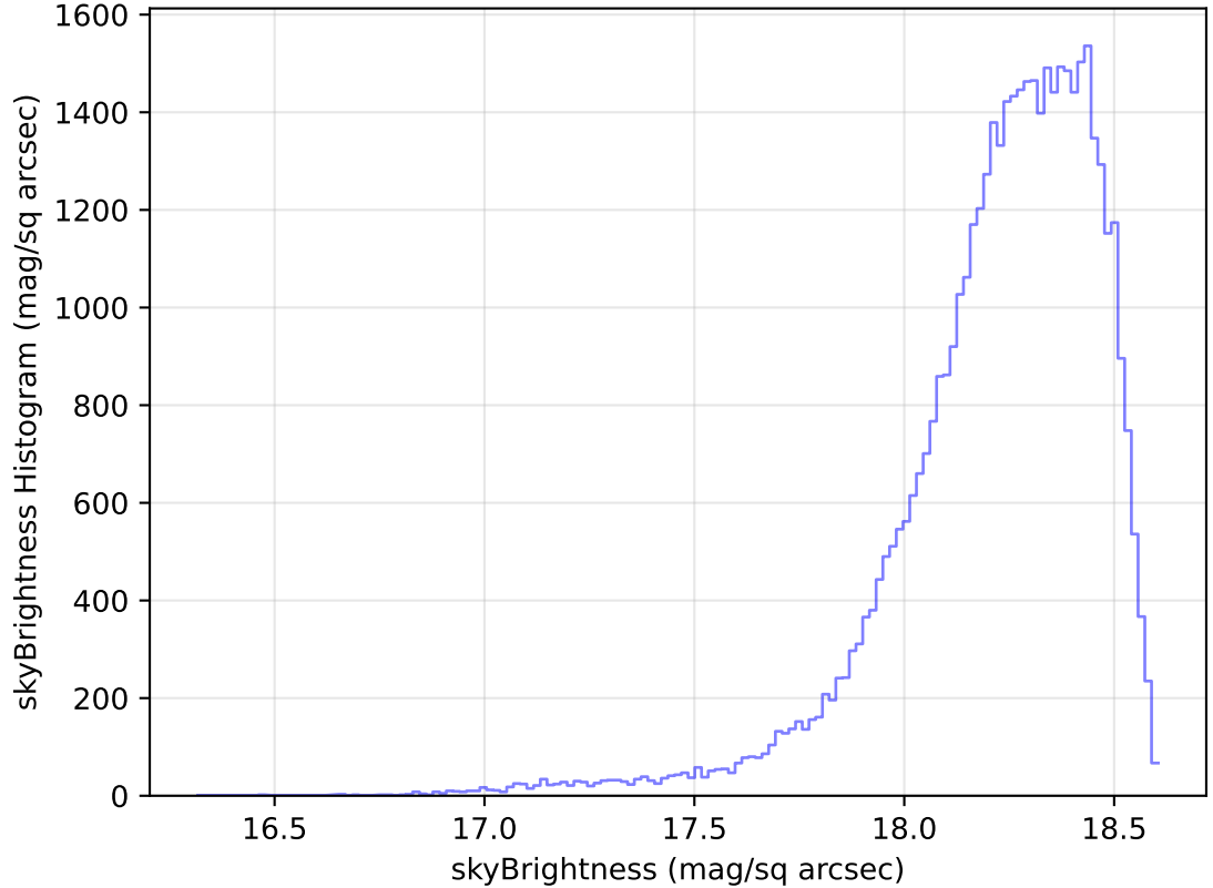
internal_u_expt38_nscale1.1v3.4_10yrs Yr 1 y band: skyBrightness Histogram
