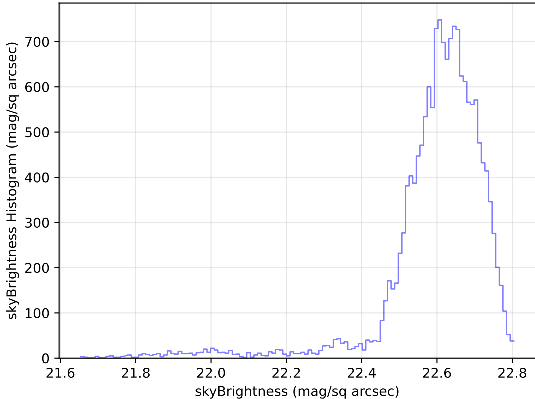
internal_u_expt38_nscale1.1v3.4_10yrs Yr 1 u band: skyBrightness Histogram
