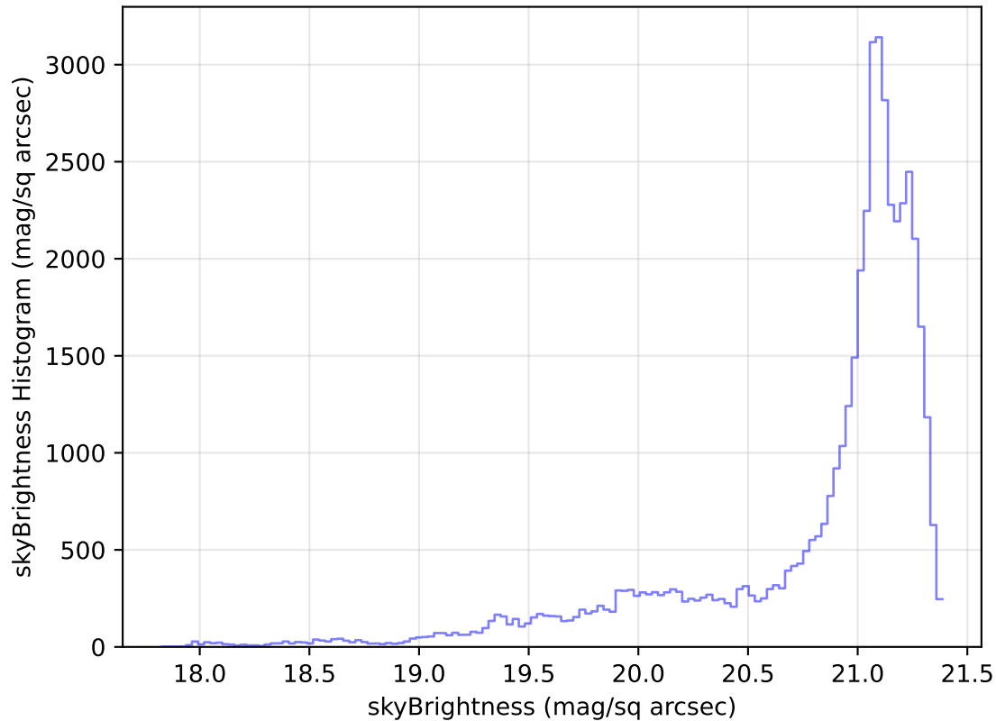
internal_u_expt38_nscale1.1v3.4_10yrs Yr 1 r band: skyBrightness Histogram
