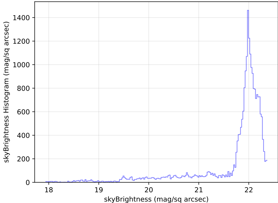
internal_u_expt38_nscale1.1v3.4_10yrs Yr 1 g band: skyBrightness Histogram
