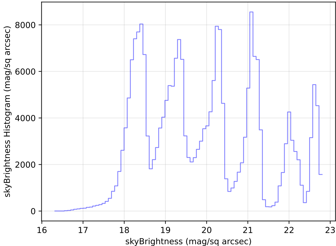
internal_u_expt38_nscale1.1v3.4_10yrs Yr 1 all bands: skyBrightness Histogram
