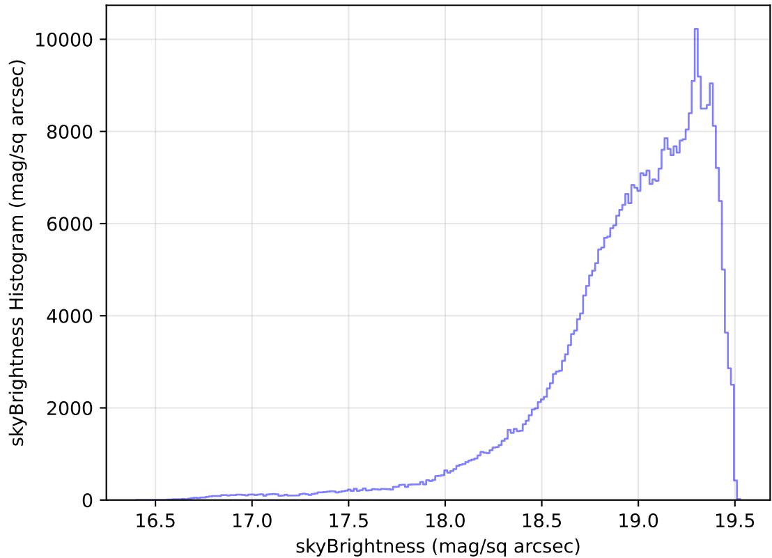
internal_u_expt38_nscale1.1v3.4_10yrs WFD z band: skyBrightness Histogram
