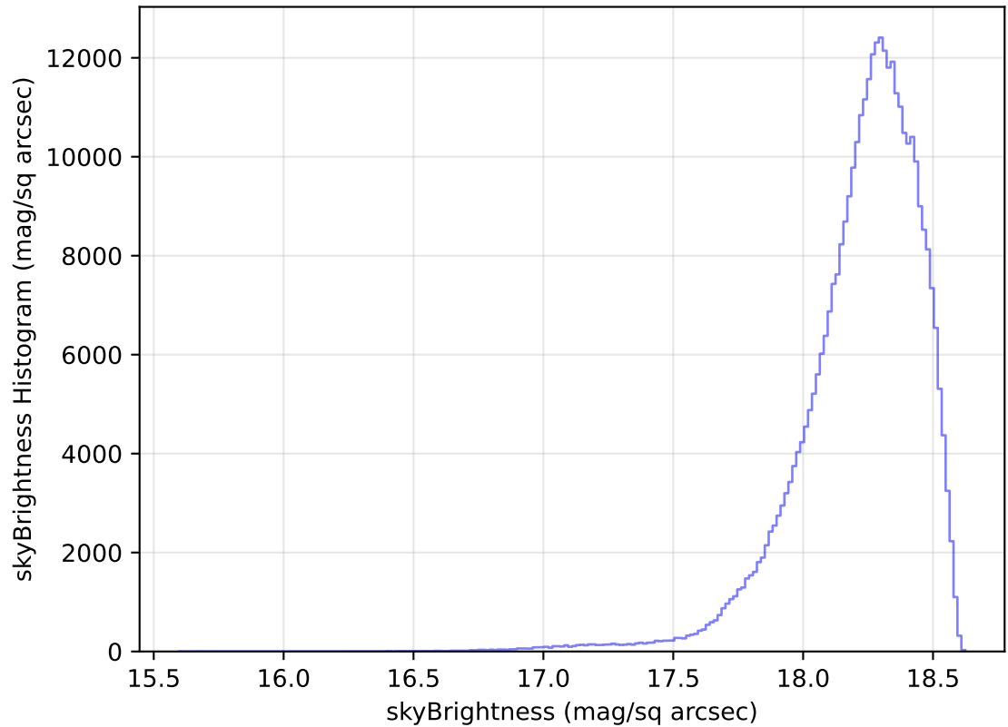
internal_u_expt38_nscale1.1v3.4_10yrs WFD y band: skyBrightness Histogram
