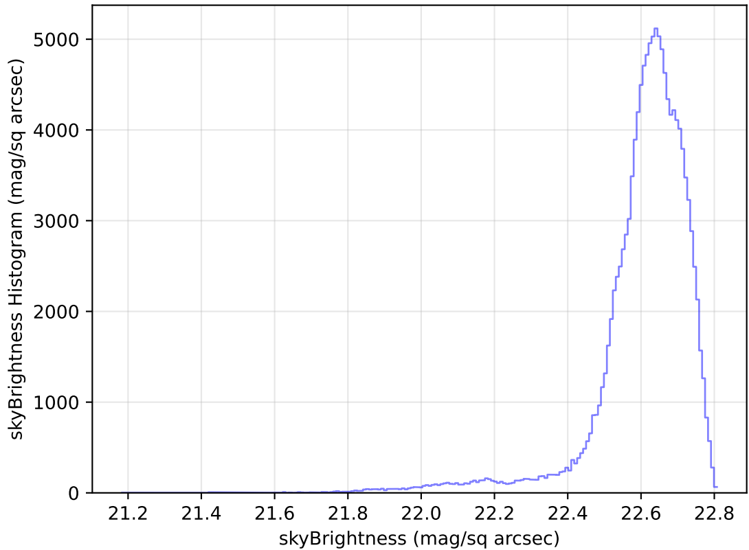
internal_u_expt38_nscale1.1v3.4_10yrs WFD u band: skyBrightness Histogram
