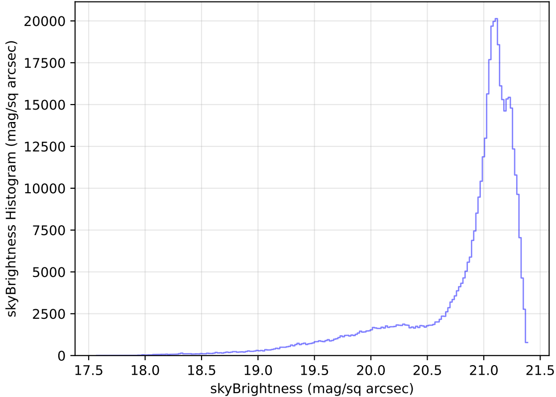
internal_u_expt38_nscale1.1v3.4_10yrs WFD r band: skyBrightness Histogram
