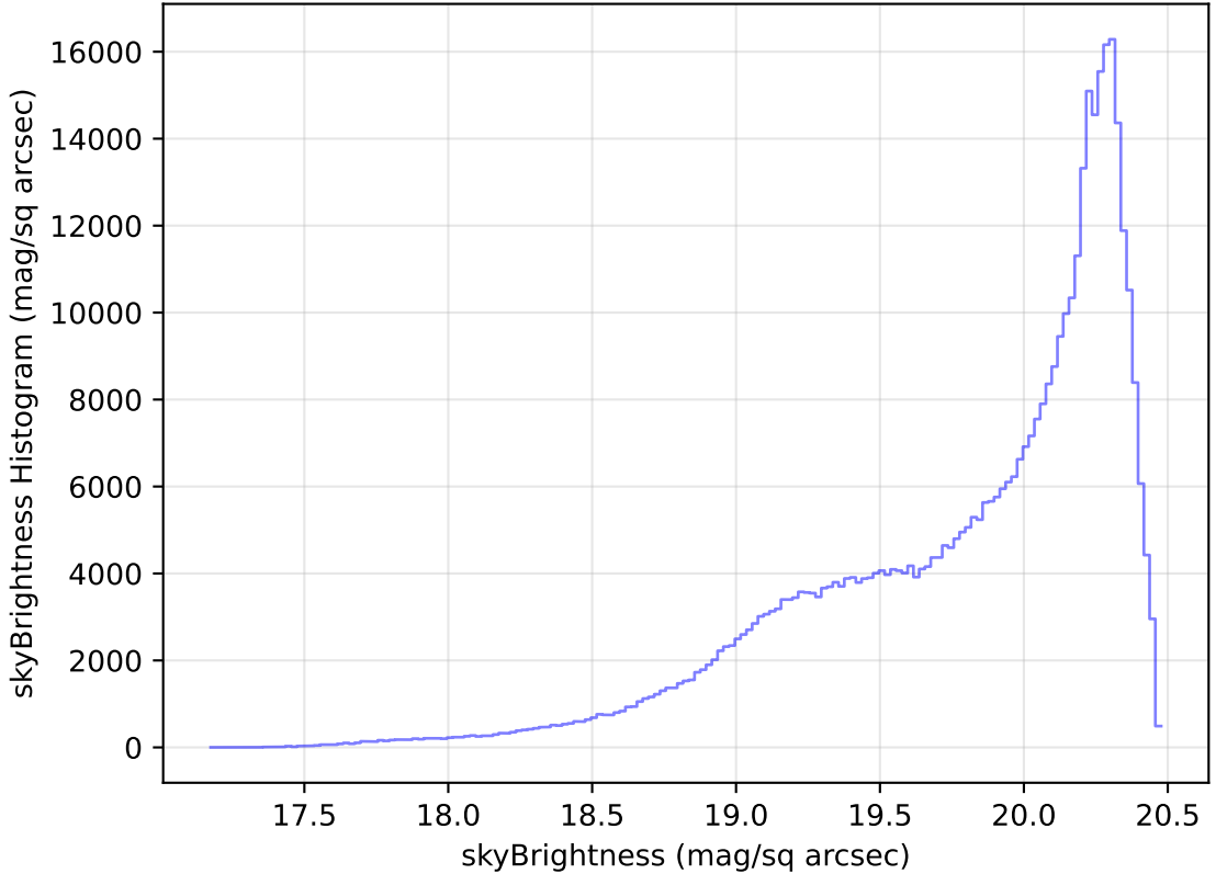
internal_u_expt38_nscale1.1v3.4_10yrs WFD i band: skyBrightness Histogram
