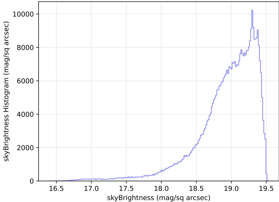
internal_u_expt38_nscale1.1v3.4_10yrs All sky z band: skyBrightness Histogram
