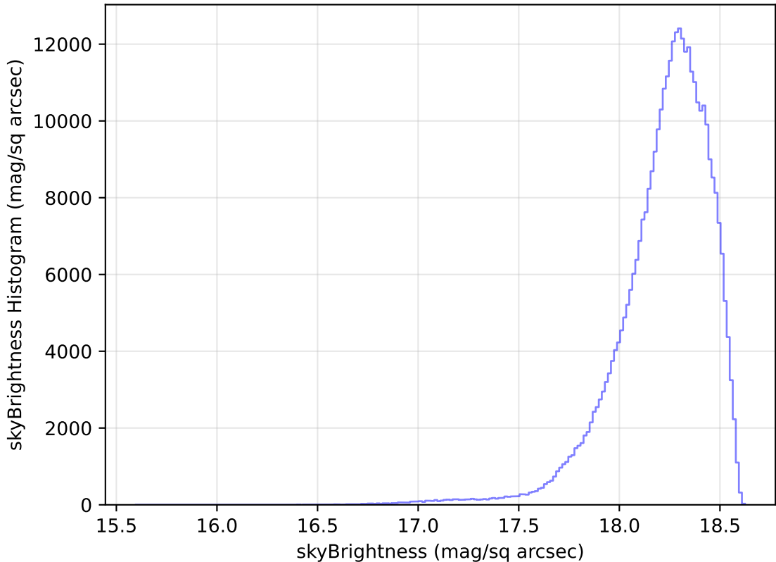
internal_u_expt38_nscale1.1v3.4_10yrs All sky y band: skyBrightness Histogram
