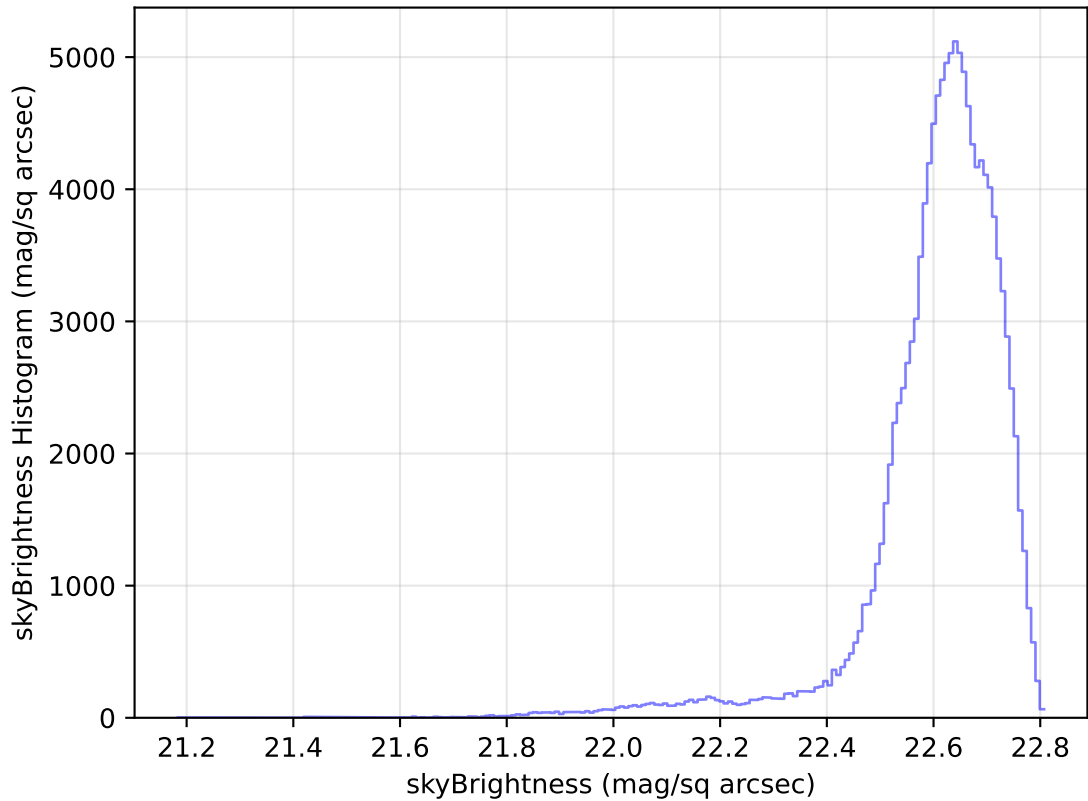
internal_u_expt38_nscale1.1v3.4_10yrs All sky u band: skyBrightness Histogram
