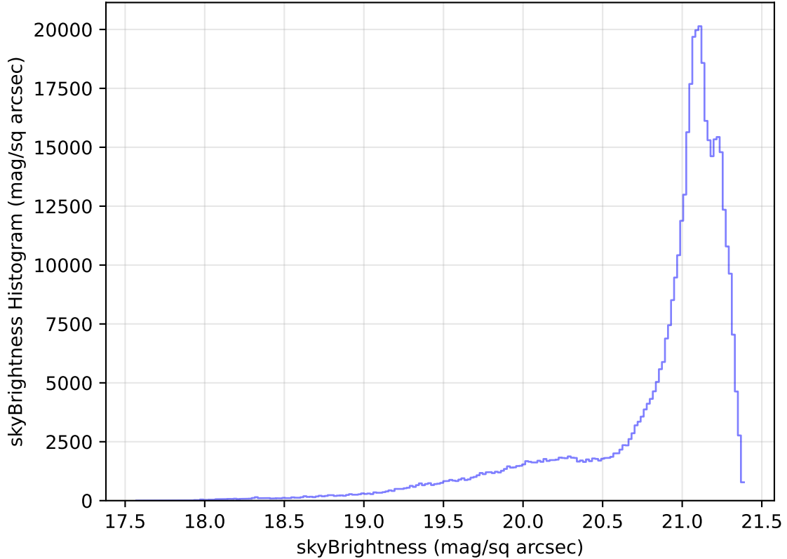
internal_u_expt38_nscale1.1v3.4_10yrs All sky r band: skyBrightness Histogram
