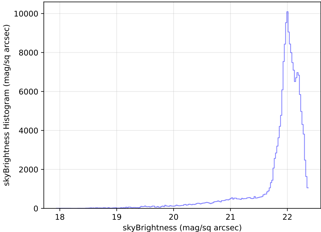
internal_u_expt38_nscale1.1v3.4_10yrs All sky g band: skyBrightness Histogram
