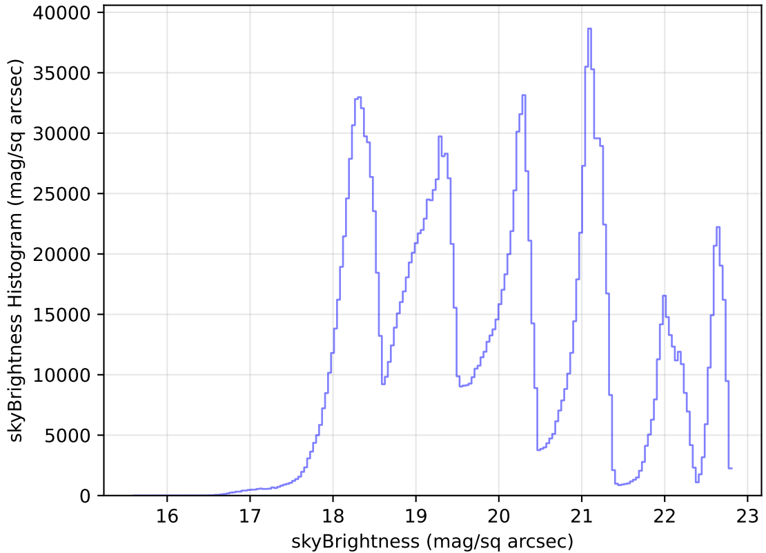
internal_u_expt38_nscale1.1v3.4_10yrs All sky all bands: skyBrightness Histogram
