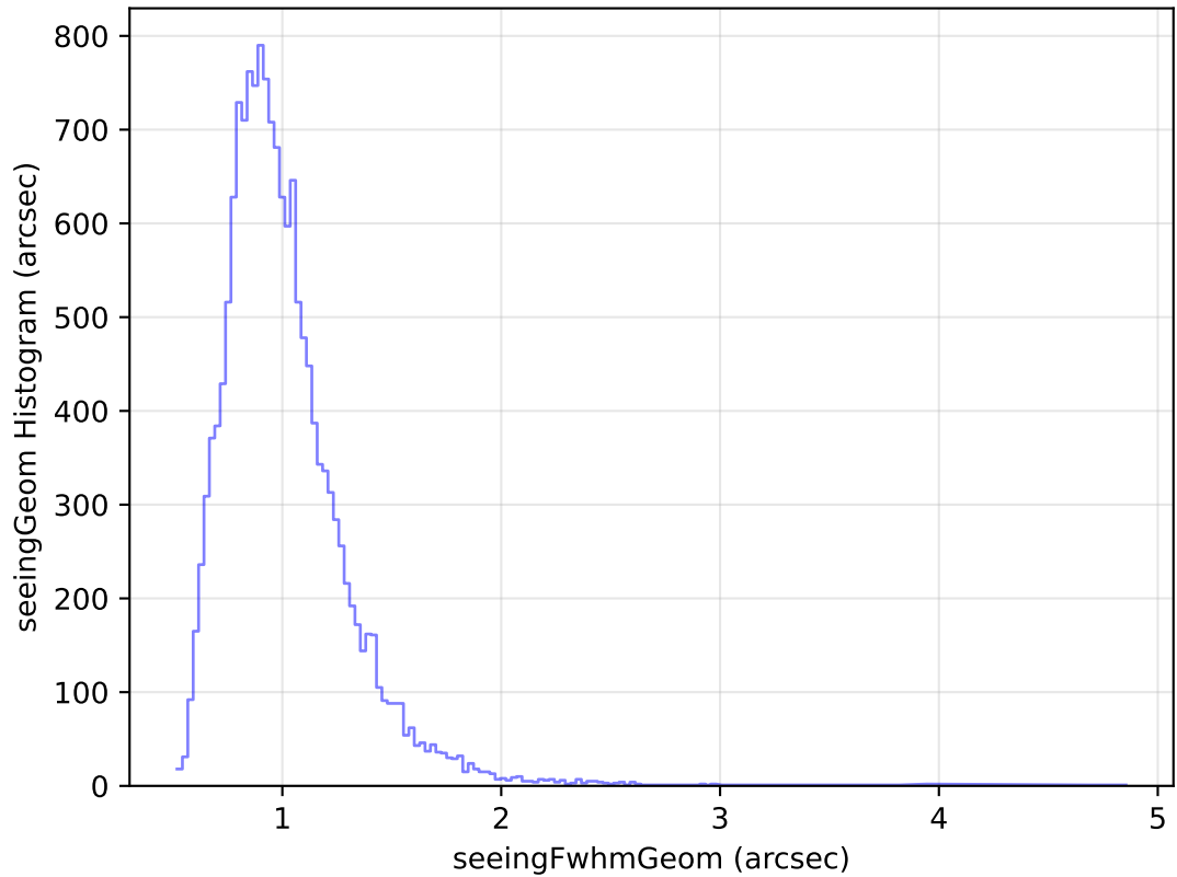
internal_u_expt38_nscale1.1v3.4_10yrs Yr 1 u band: seeingGeom Histogram
