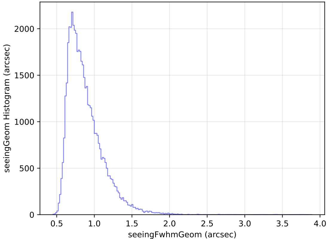
internal_u_expt38_nscale1.1v3.4_10yrs Yr 1 r band: seeingGeom Histogram
