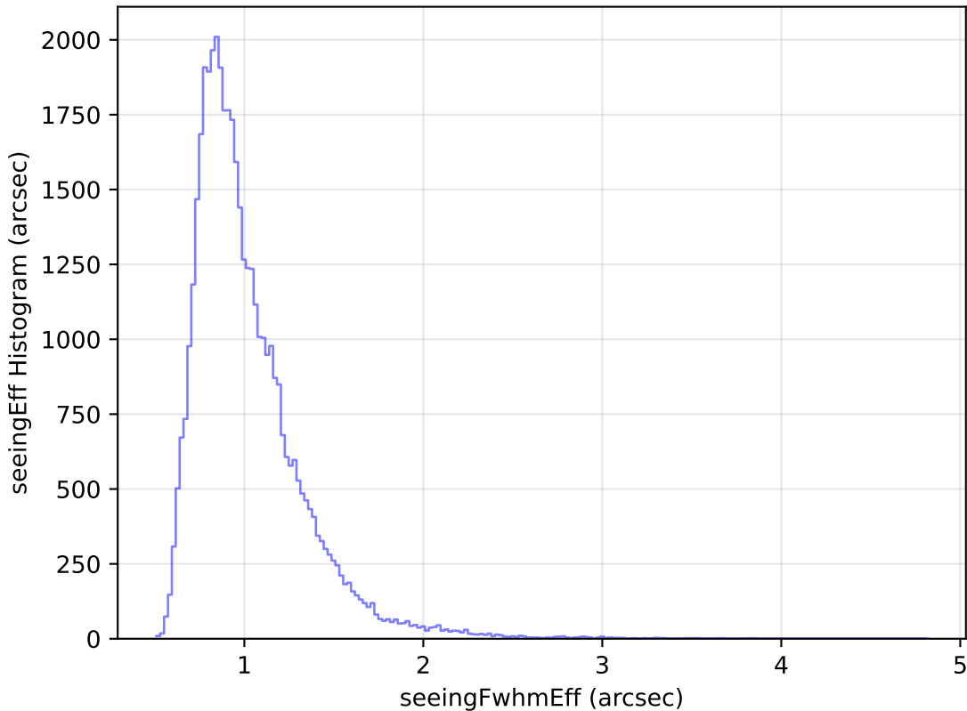
internal_u_expt38_nscale1.1v3.4_10yrs Yr 1 z band: seeingEff Histogram
