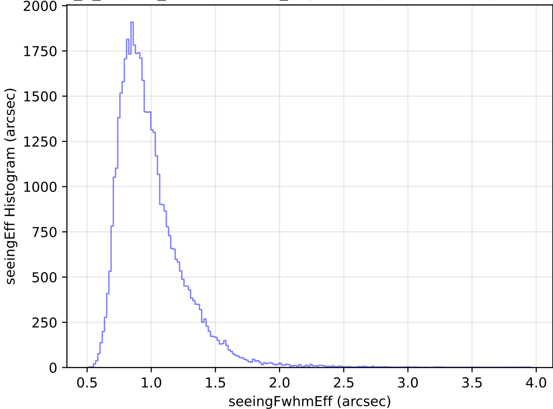
internal_u_expt38_nscale1.1v3.4_10yrs Yr 1 y band: seeingEff Histogram
