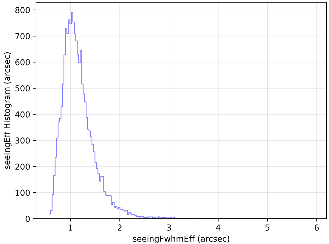
internal_u_expt38_nscale1.1v3.4_10yrs Yr 1 u band: seeingEff Histogram
