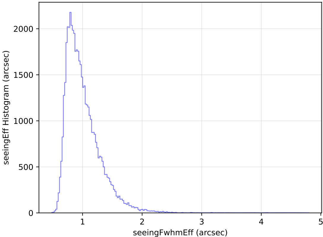
internal_u_expt38_nscale1.1v3.4_10yrs Yr 1 r band: seeingEff Histogram
