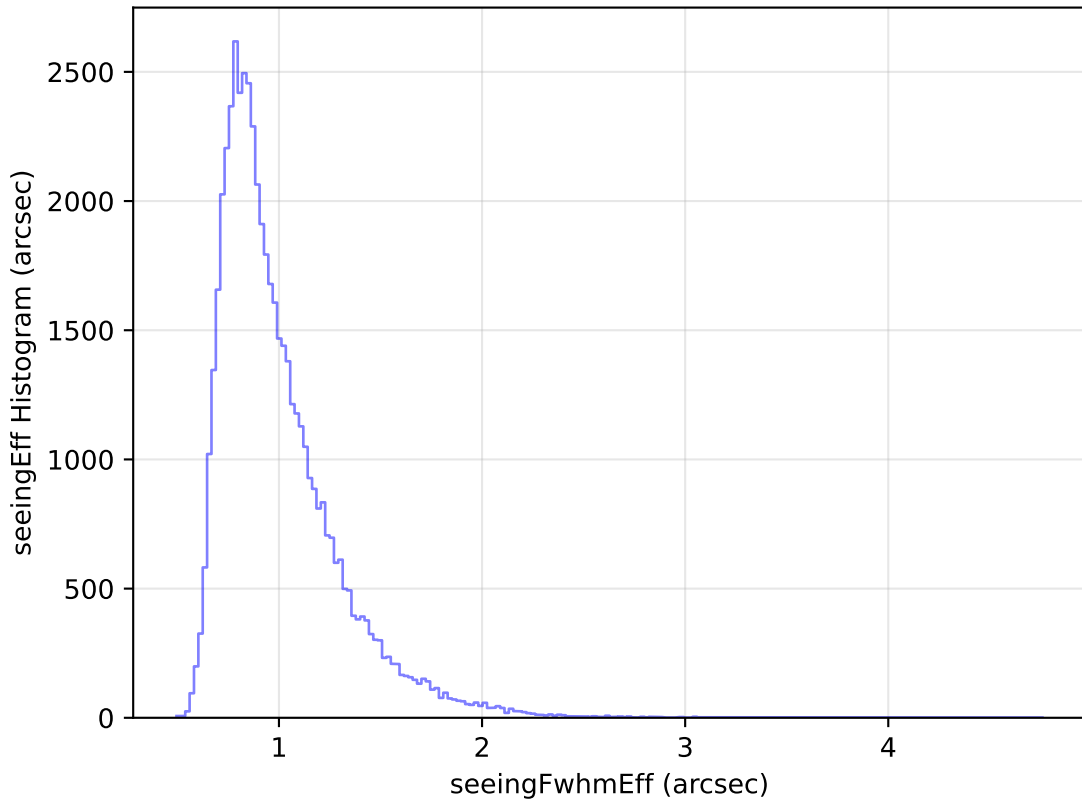
internal_u_expt38_nscale1.1v3.4_10yrs Yr 1 i band: seeingEff Histogram
