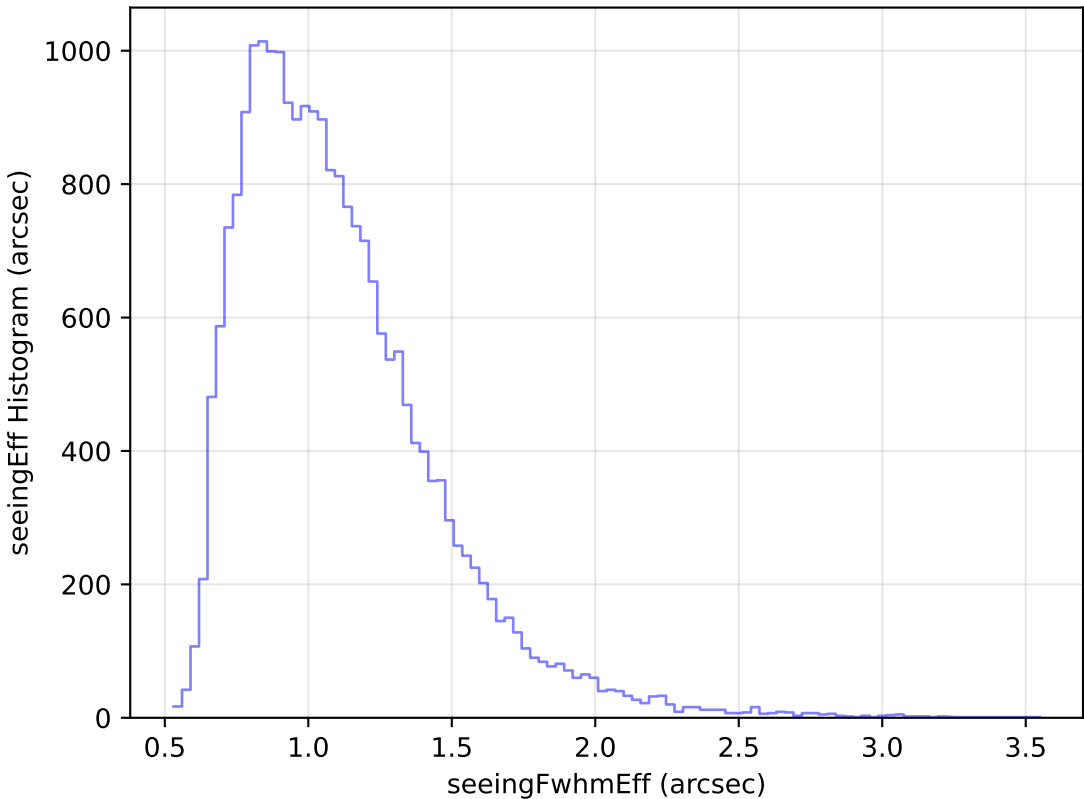
internal_u_expt38_nscale1.1v3.4_10yrs Yr 1 g band: seeingEff Histogram
