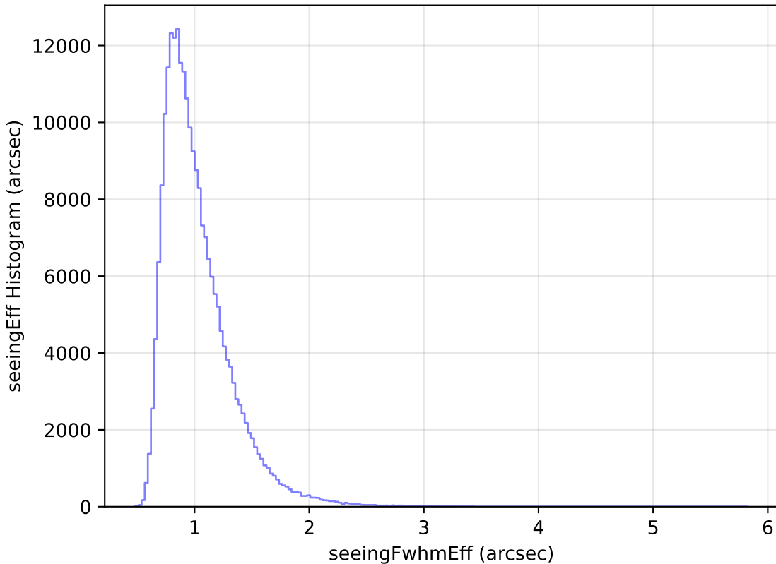
internal_u_expt38_nscale1.1v3.4_10yrs Yr 1 all bands: seeingEff Histogram
