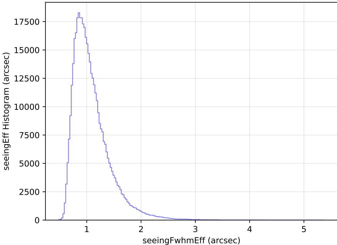
internal_u_expt38_nscale1.1v3.4_10yrs WFD z band: seeingEff Histogram
