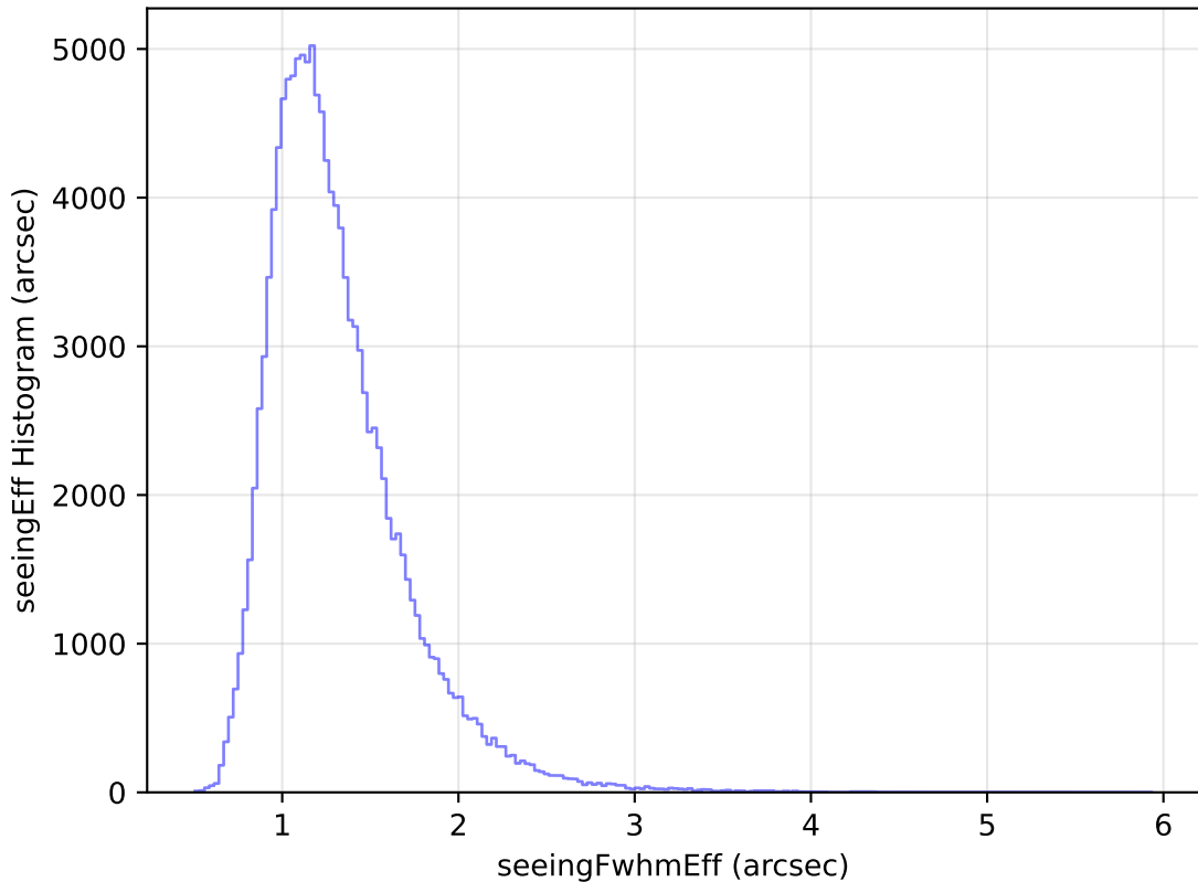
internal_u_expt38_nscale1.1v3.4_10yrs WFD u band: seeingEff Histogram
