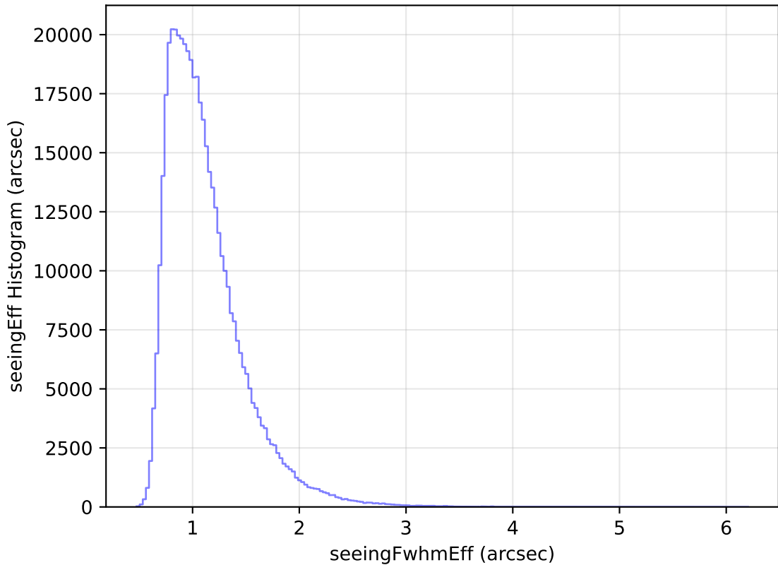
internal_u_expt38_nscale1.1v3.4_10yrs WFD r band: seeingEff Histogram
