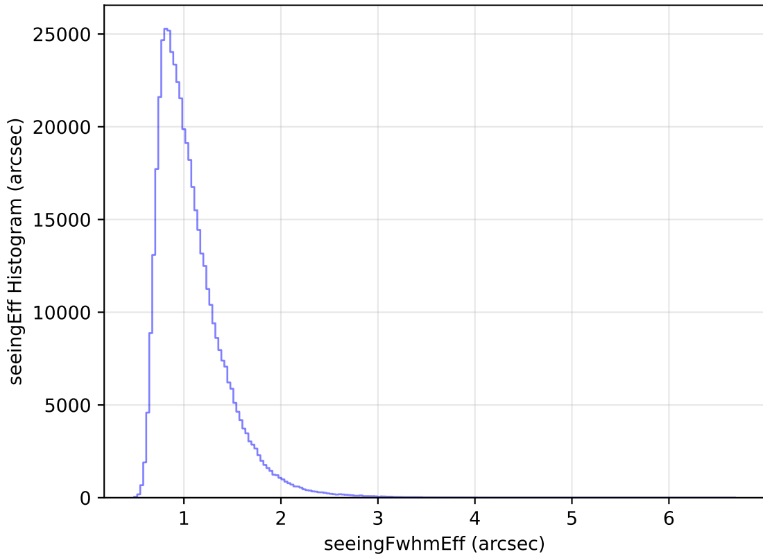
internal_u_expt38_nscale1.1v3.4_10yrs WFD i band: seeingEff Histogram
