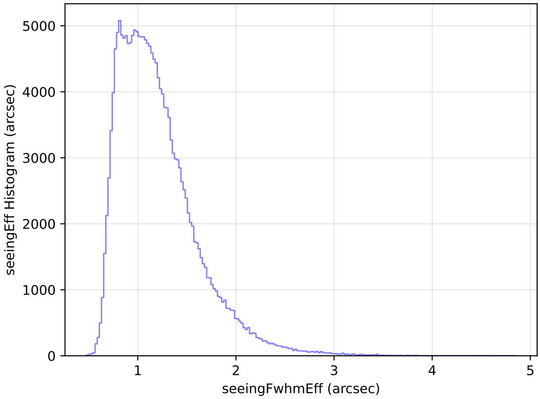
internal_u_expt38_nscale1.1v3.4_10yrs WFD g band: seeingEff Histogram
