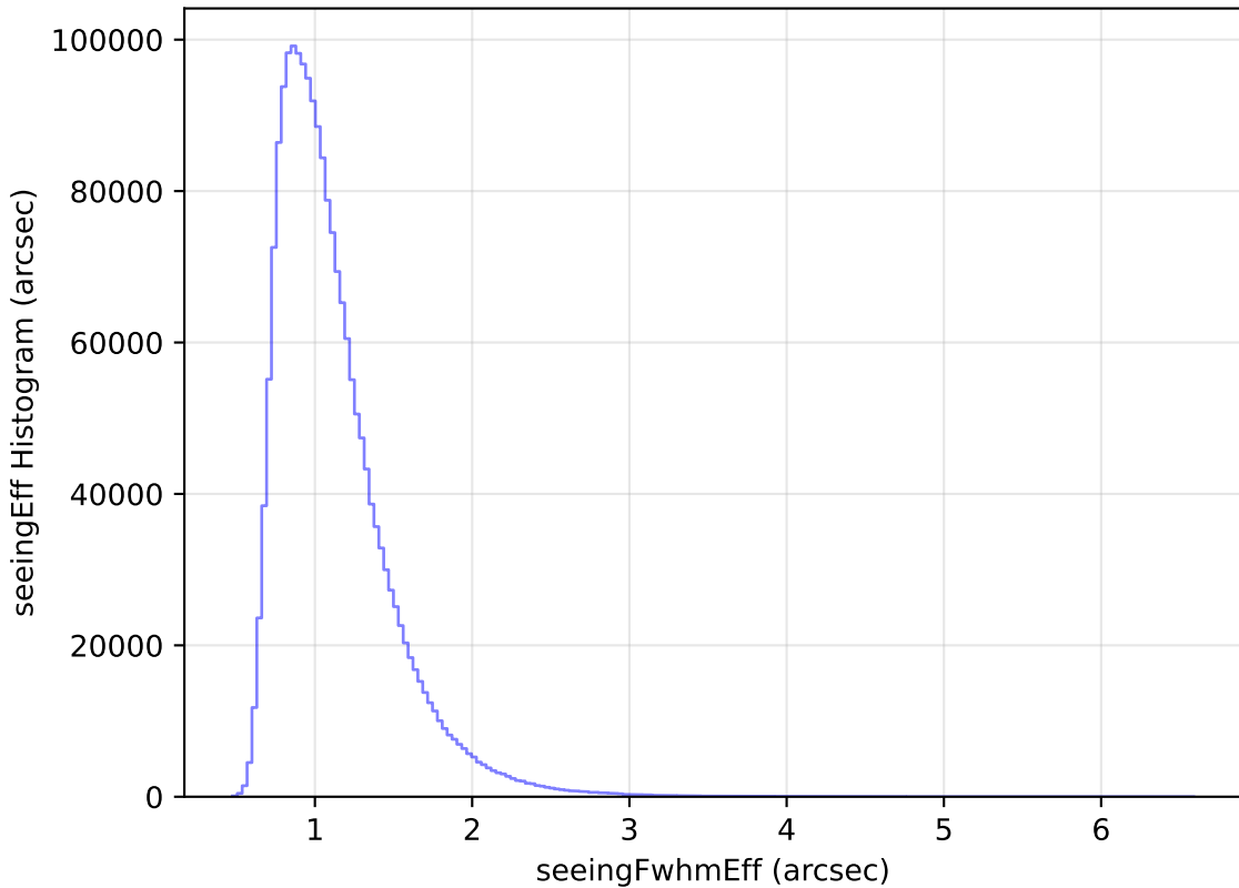
internal_u_expt38_nscale1.1v3.4_10yrs WFD all bands: seeingEff Histogram
