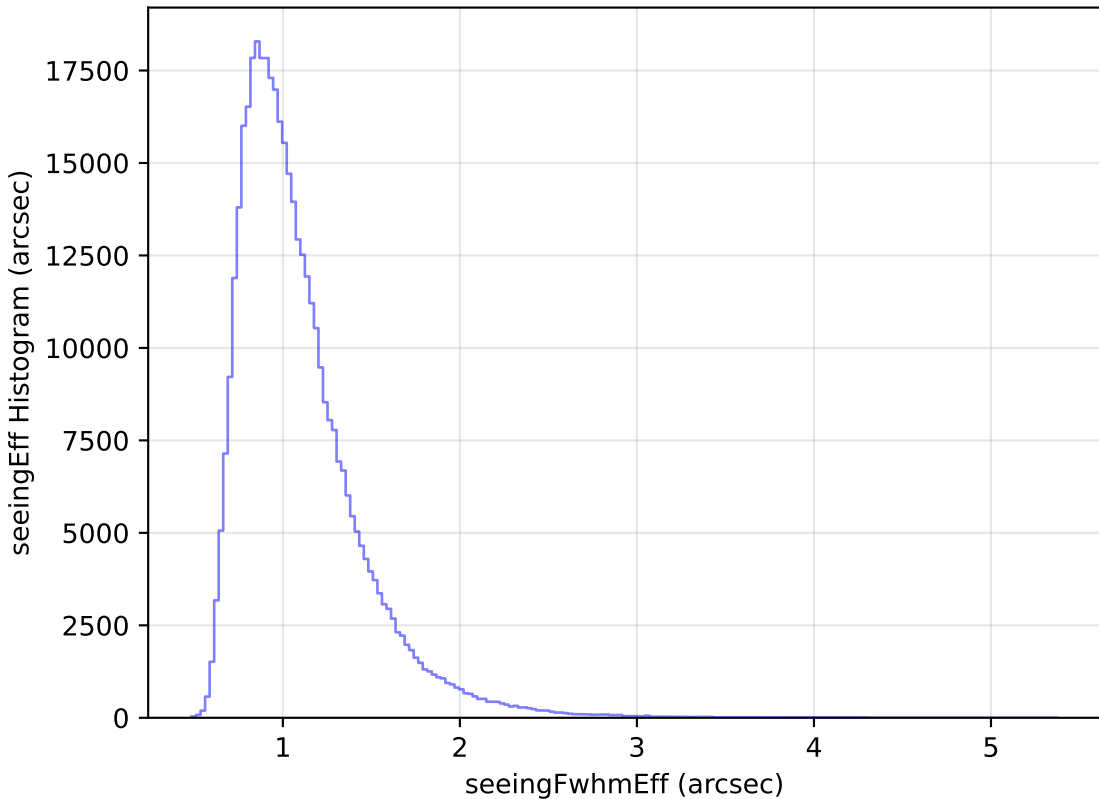
internal_u_expt38_nscale1.1v3.4_10yrs All sky z band: seeingEff Histogram
