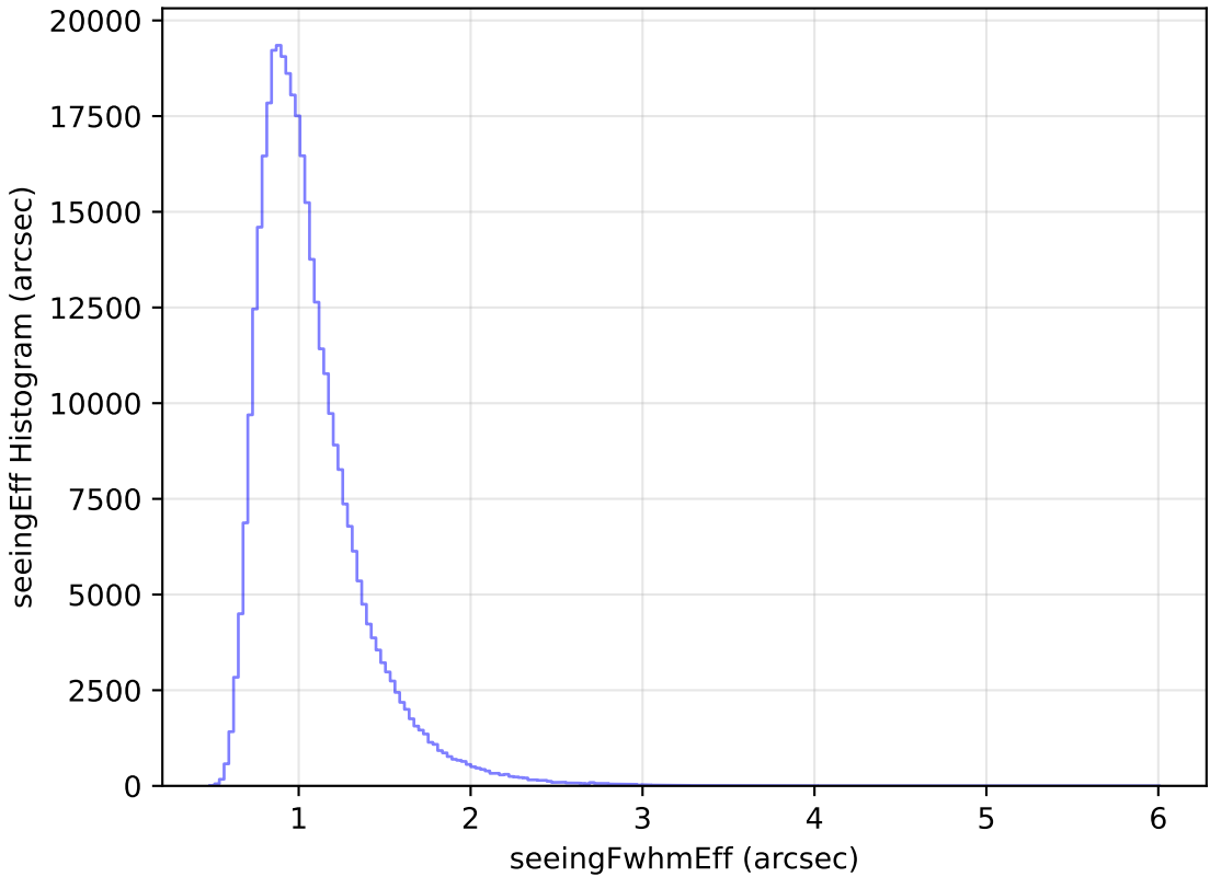
internal_u_expt38_nscale1.1v3.4_10yrs All sky y band: seeingEff Histogram
