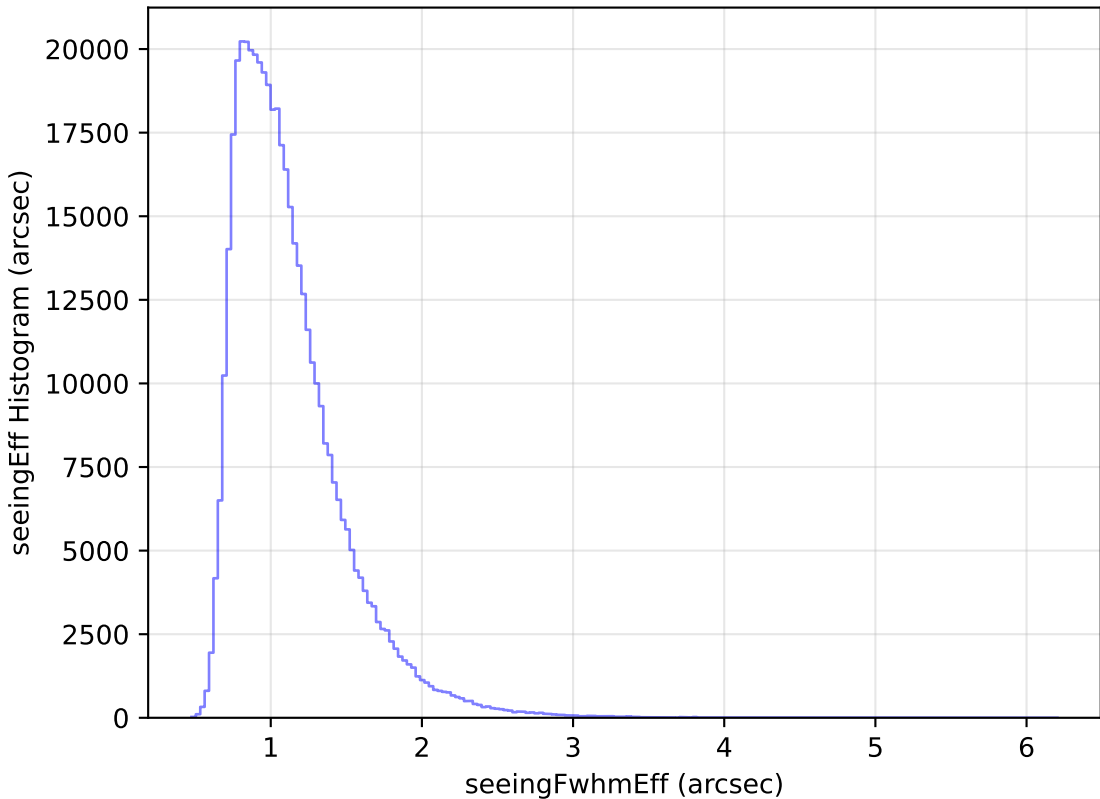
internal_u_expt38_nscale1.1v3.4_10yrs All sky r band: seeingEff Histogram
