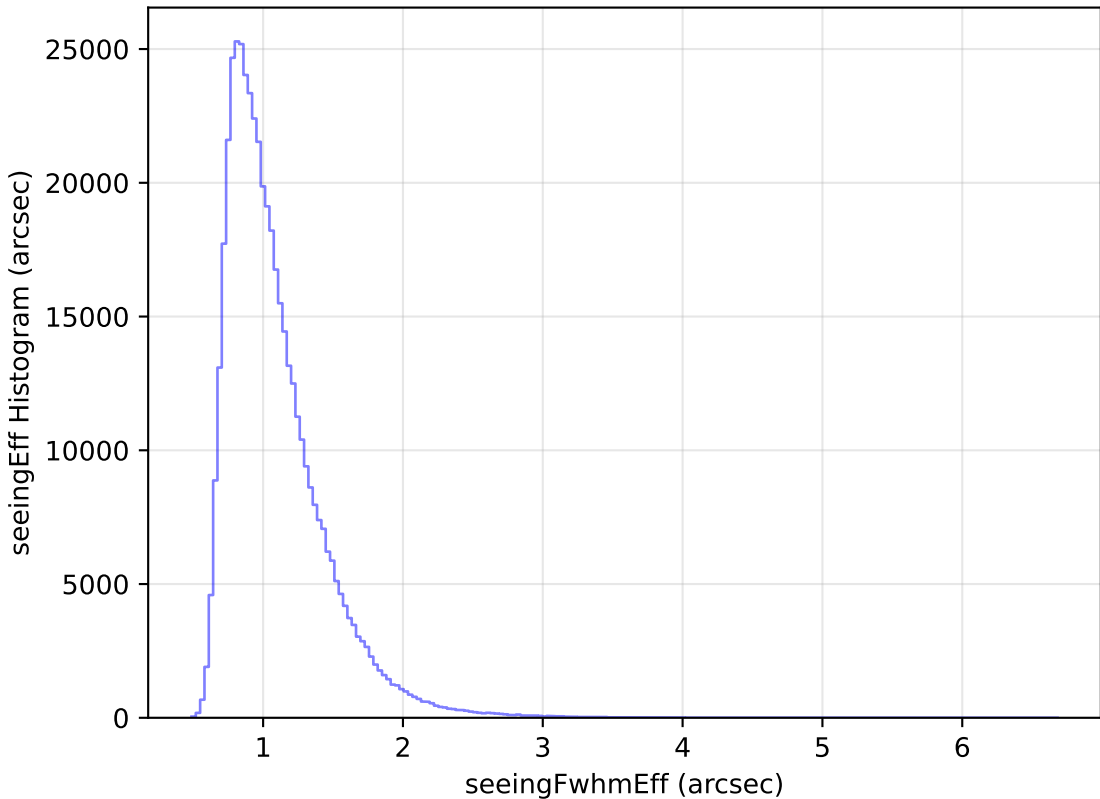
internal_u_expt38_nscale1.1v3.4_10yrs All sky i band: seeingEff Histogram
