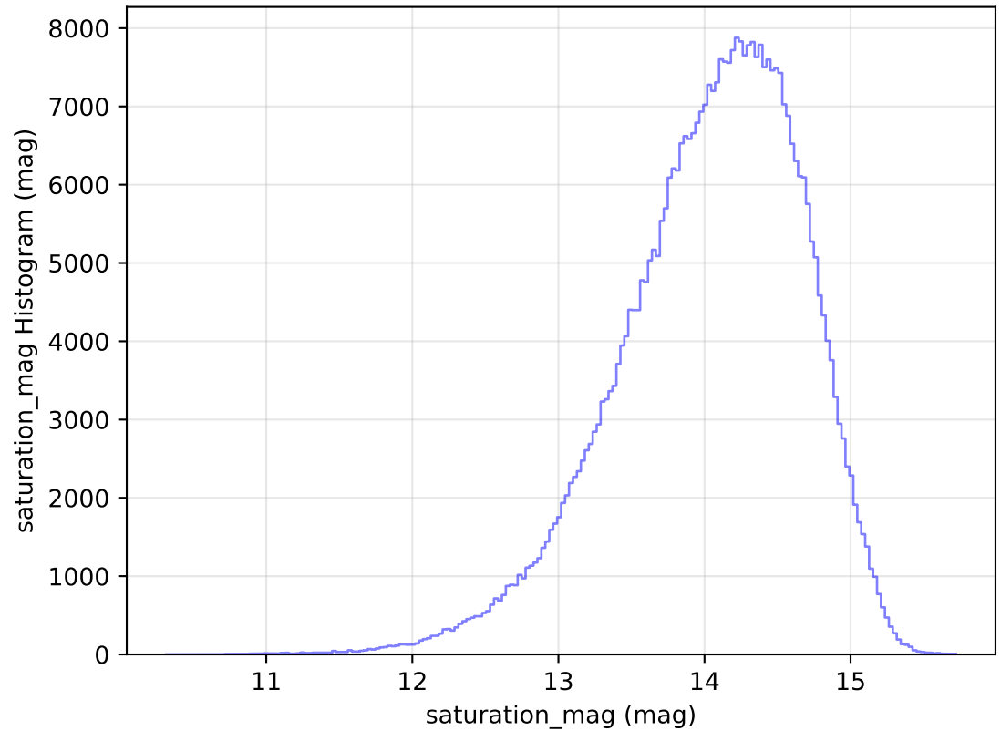
internal_u_expt38_nscale1.1v3.4_10yrs WFD z band: saturation_mag Histogram
